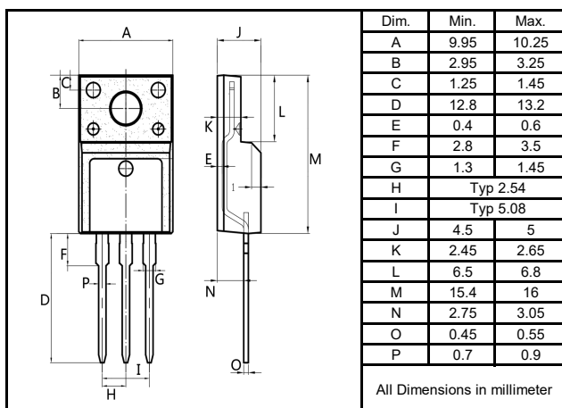
TO-220F
