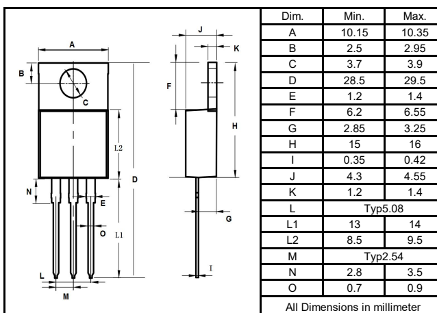
TO-220AB
